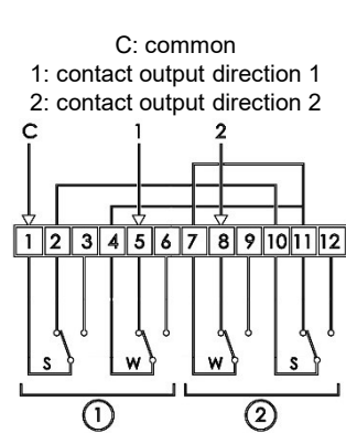
Limit switch wiring diagram
